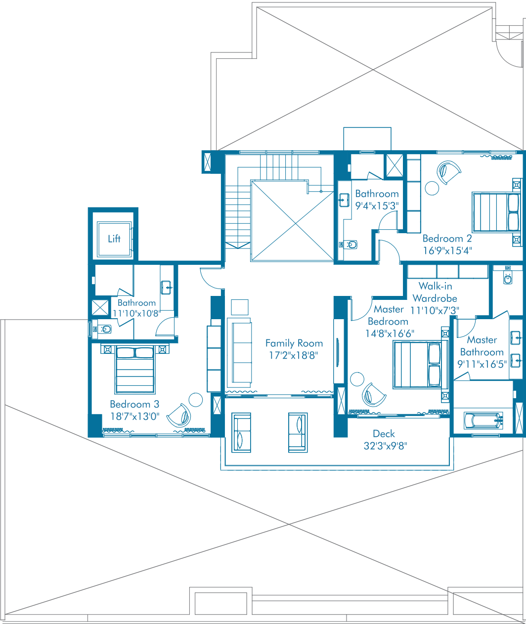
UPPER FLOOR
