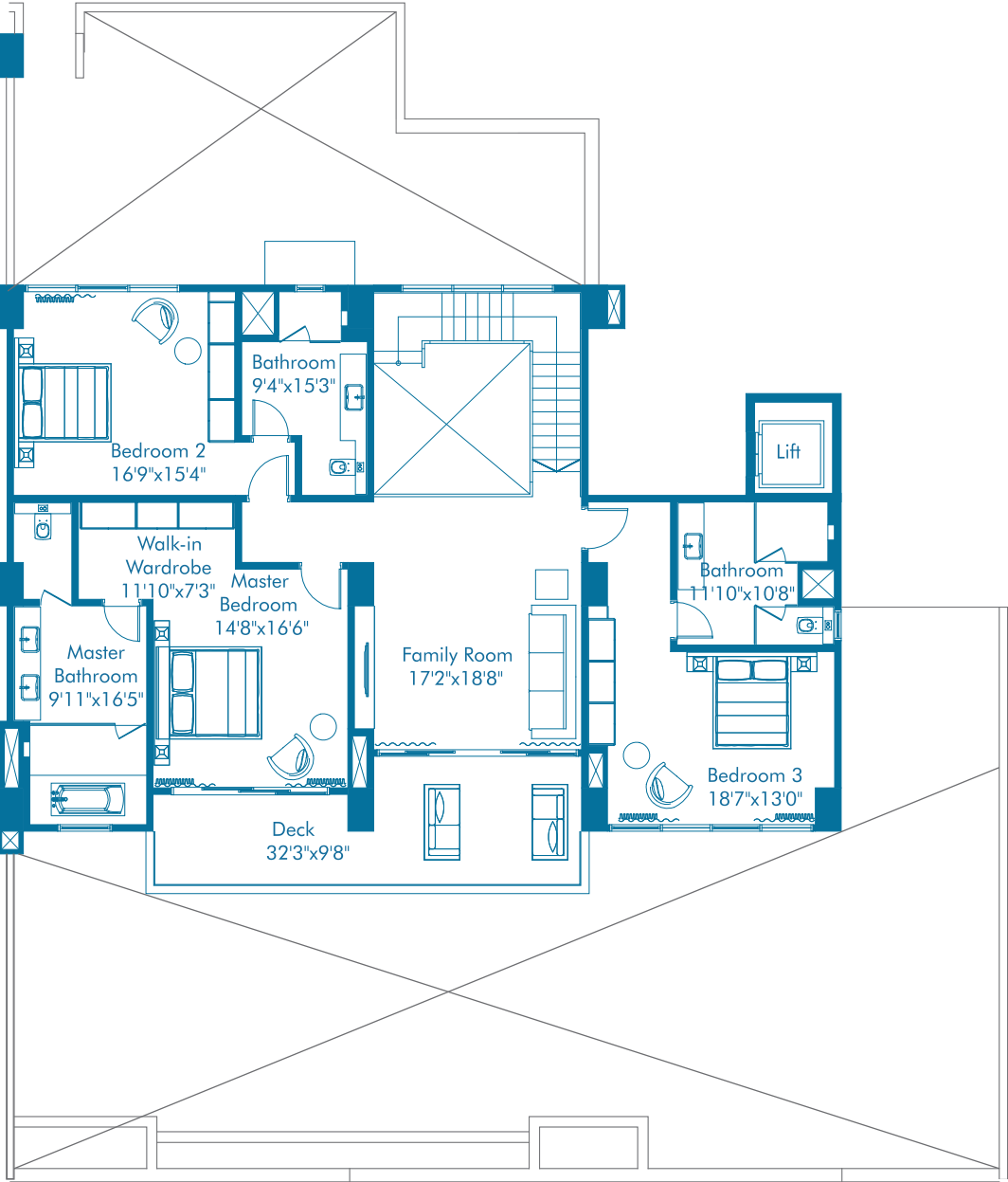
UPPER FLOOR
