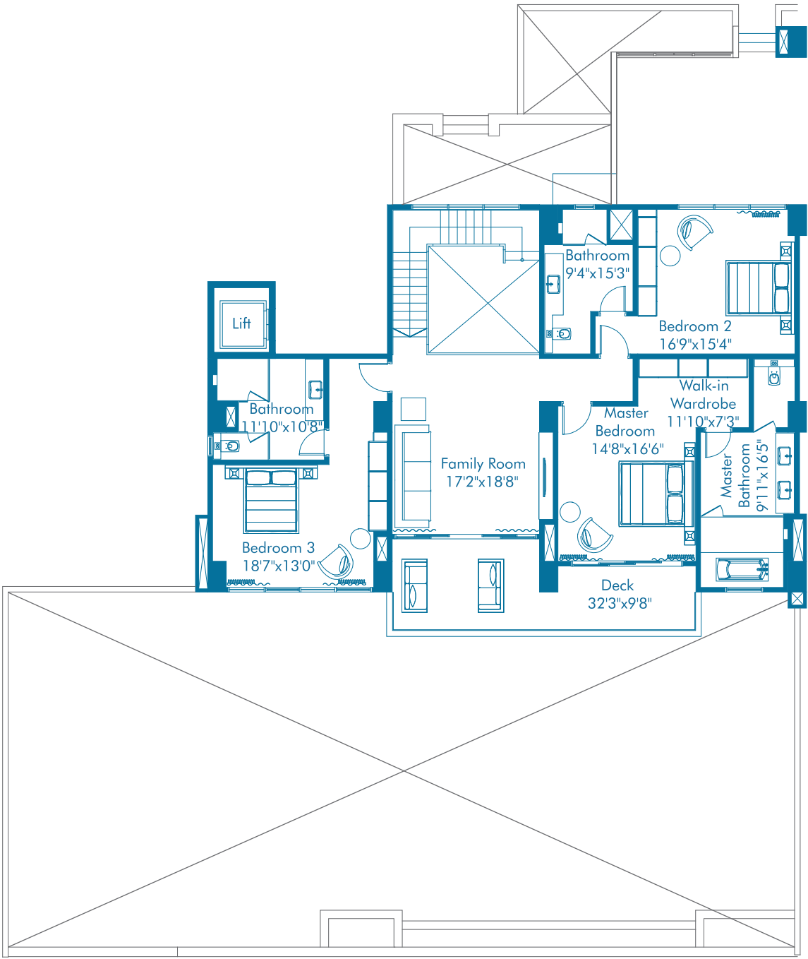
UPPER FLOOR
