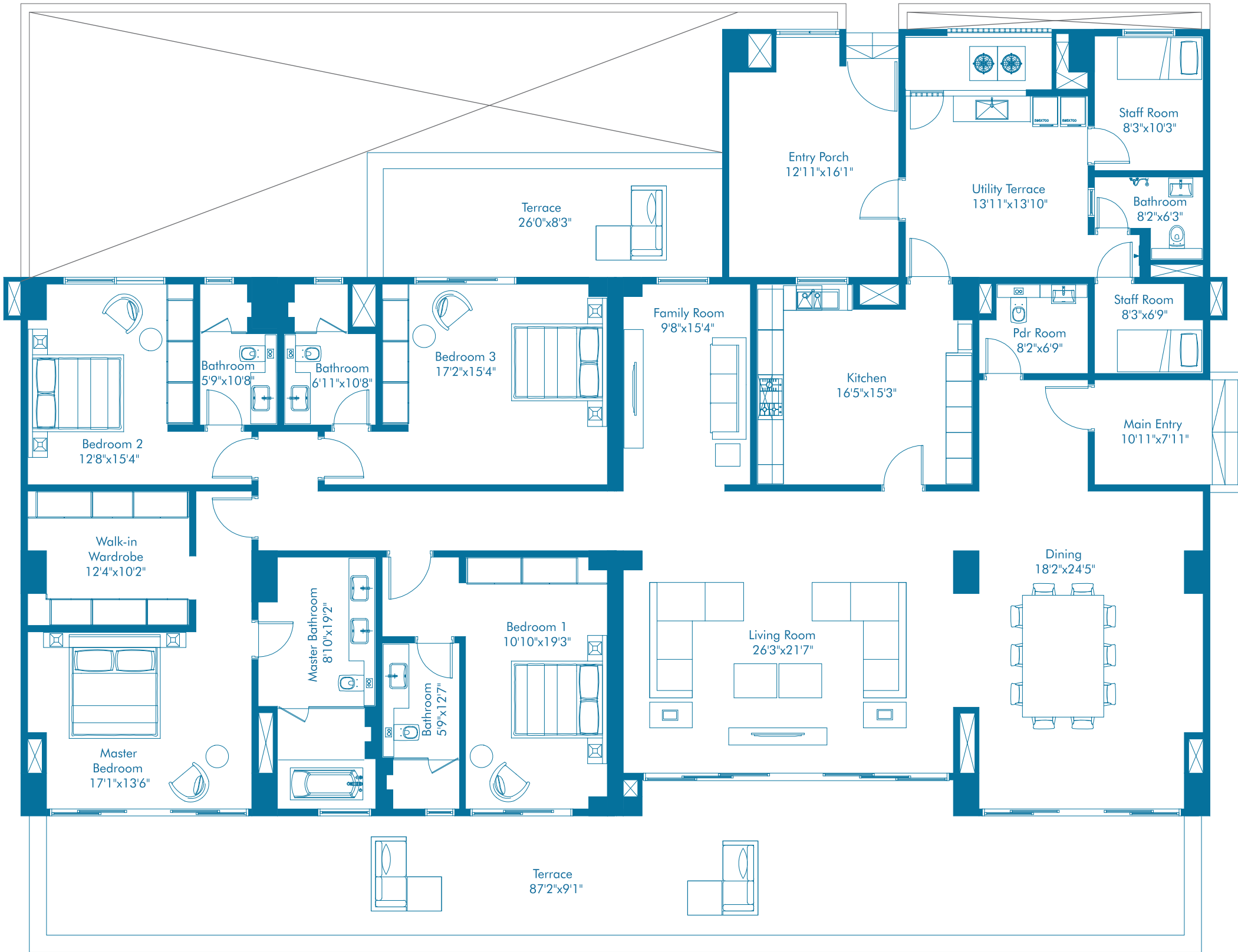
KEY PLAN
